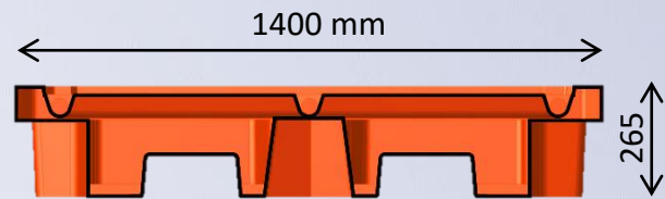
Front Elevation - Cross Section
