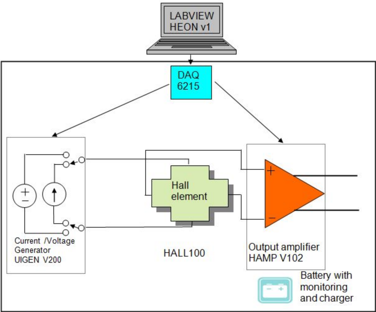
Figure 1: Block diagram of the system "Senis HEON2008 v1"
