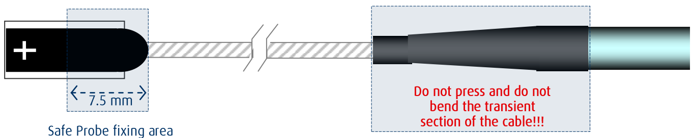
Figure 3. Safe fixing area of the P Probe head
