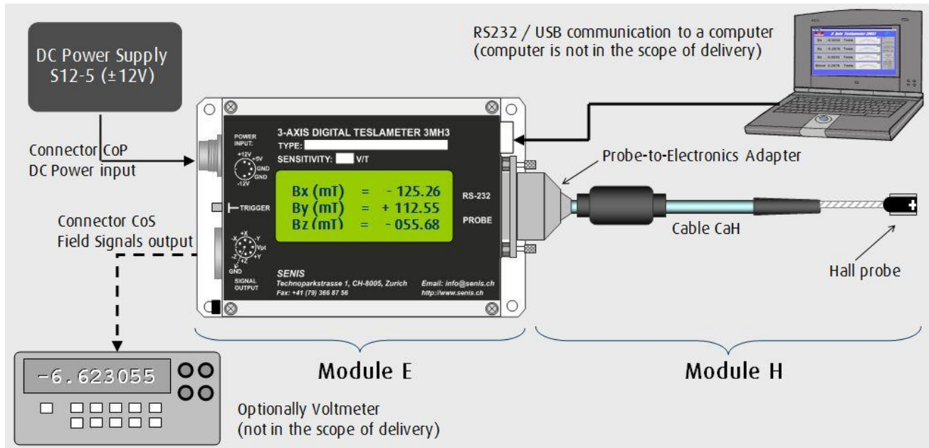
Figure 2. Structure of the high-accuracy Magnetic Field Teslameter with fully integrated Hall Probe: - Module H, consisting of the Hall Probe and the CaH Cable; - Module E, analog and digital electronics for signal conditioning.
