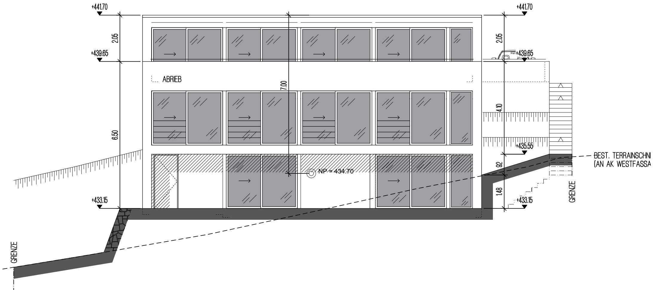
FASSADE WEST (W-W)
